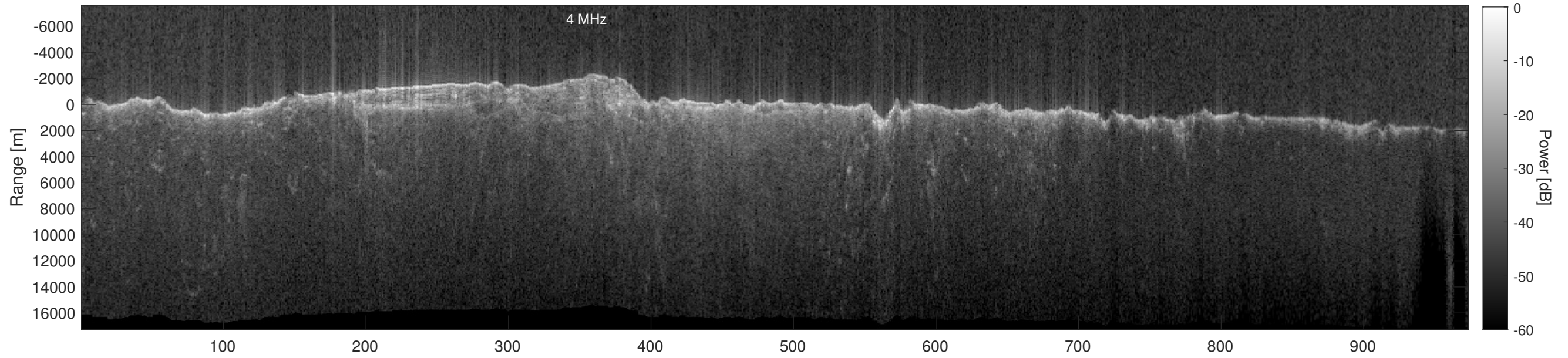
Orbit 8592, Depth-Corrected Cluttergram
