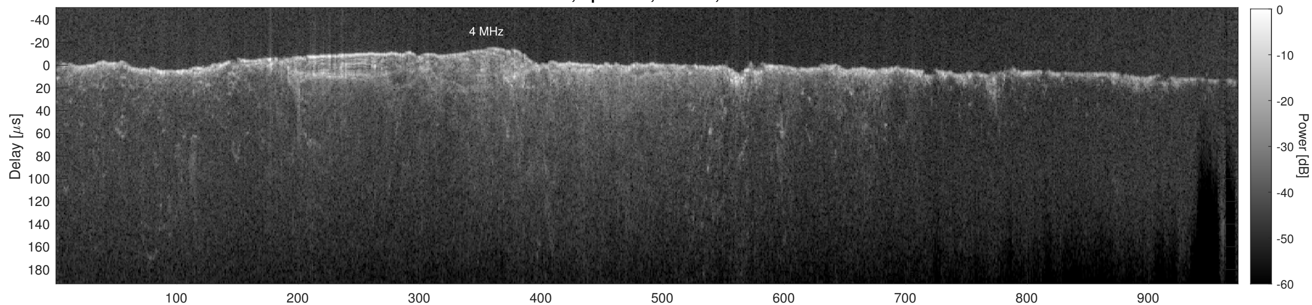
Orbit 8592, Cluttergram
