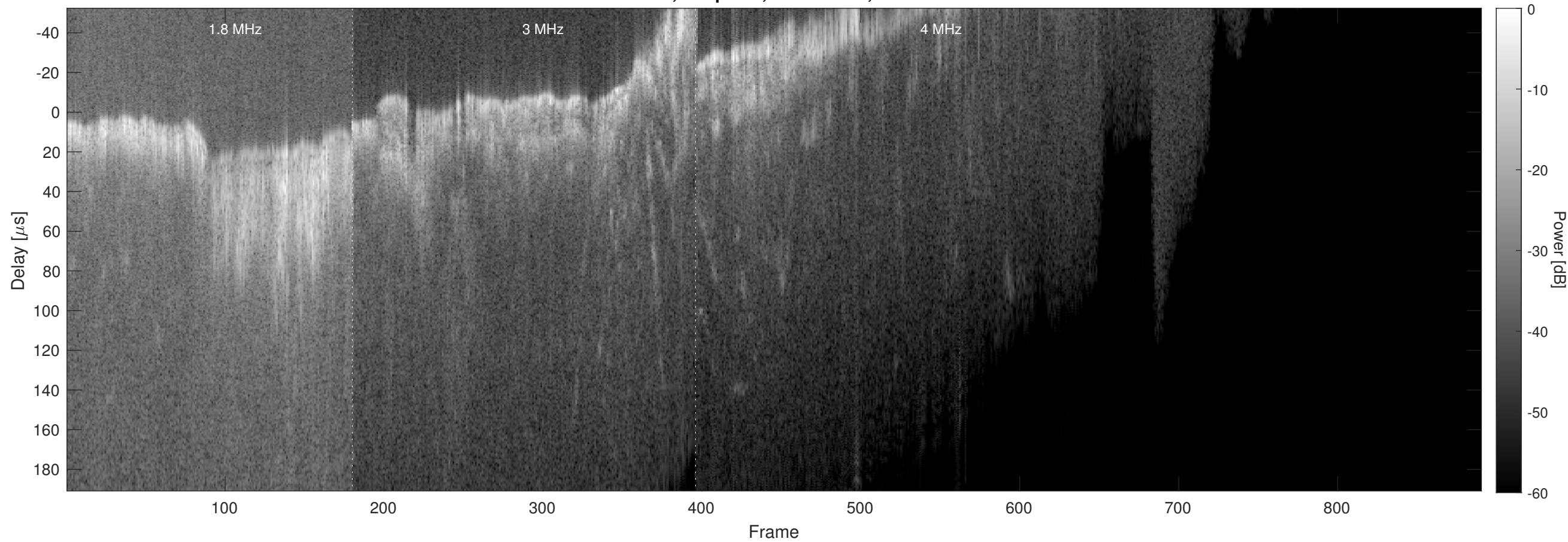
Orbit 8594, Chapman, No Window, Channel 2
