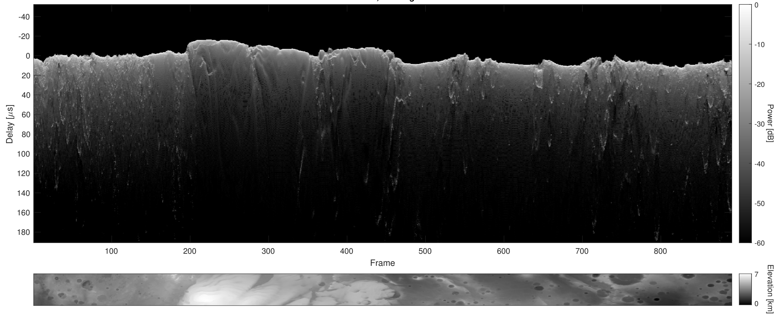
Orbit 8594, Cluttergram
