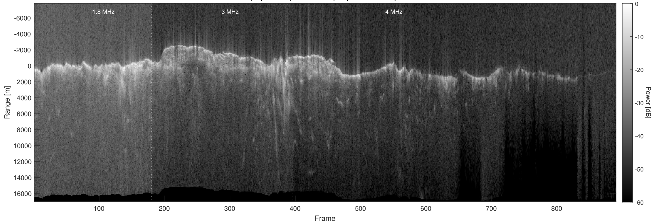
Orbit 8594, Optimized, No Window, Depth-Corrected, Channel 2
