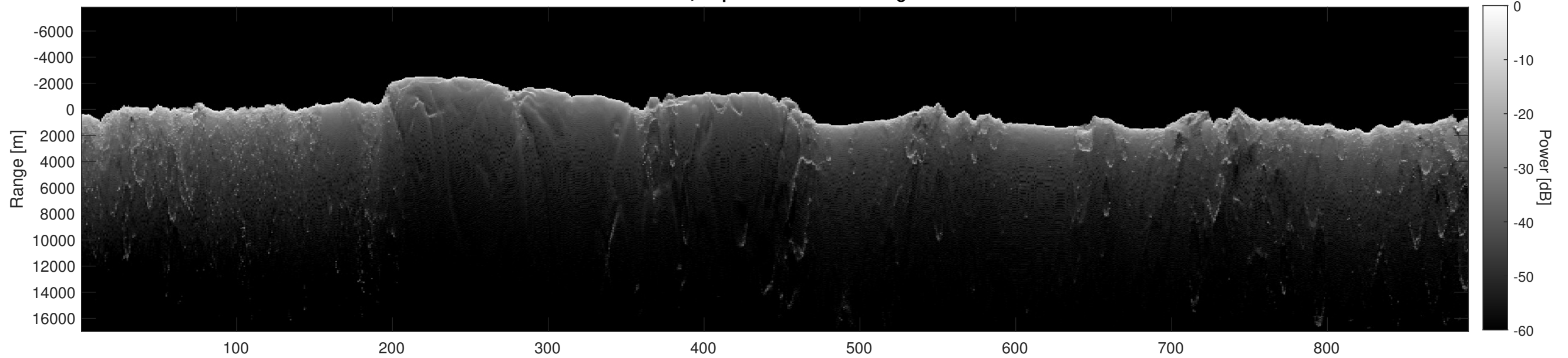
Orbit 8594, Depth-Corrected Cluttergram
