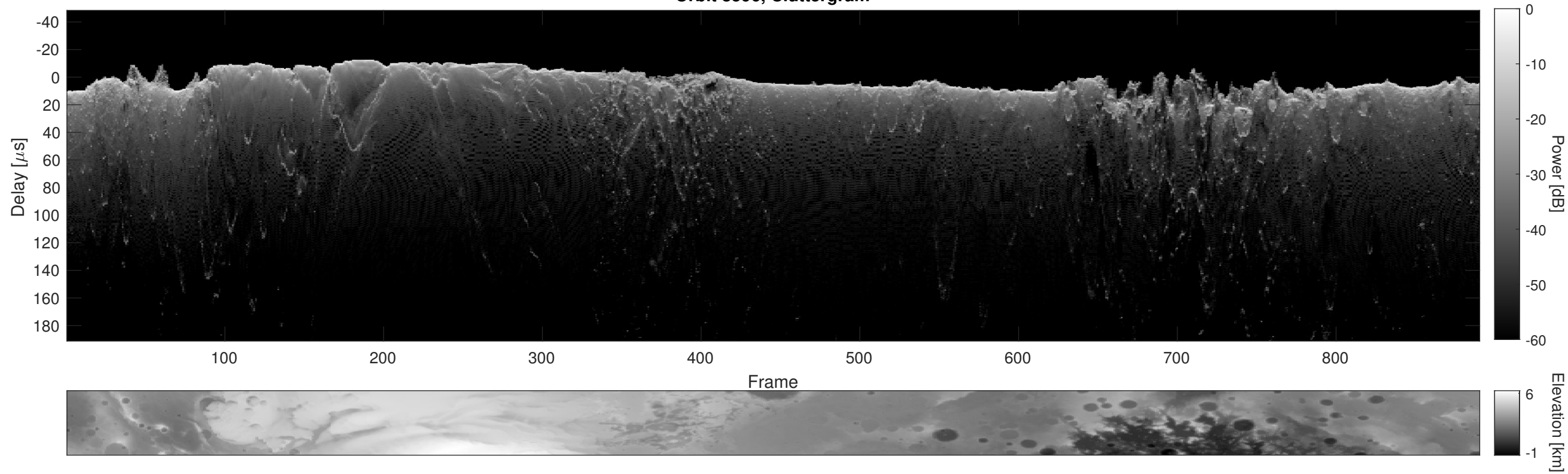
Orbit 8596, Cluttergram
