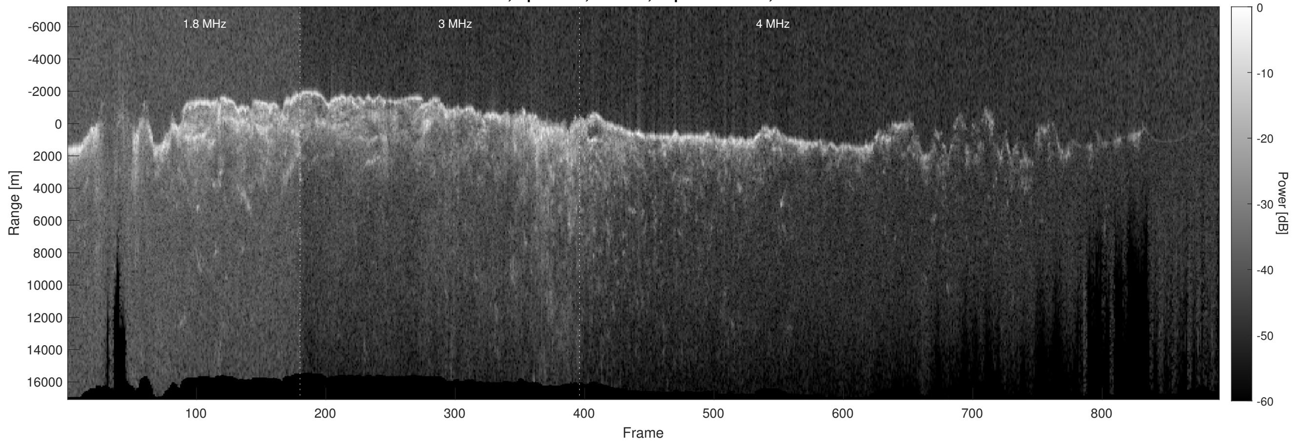
Orbit 8596, Optimized, Window, Depth-Corrected, Channel 2
