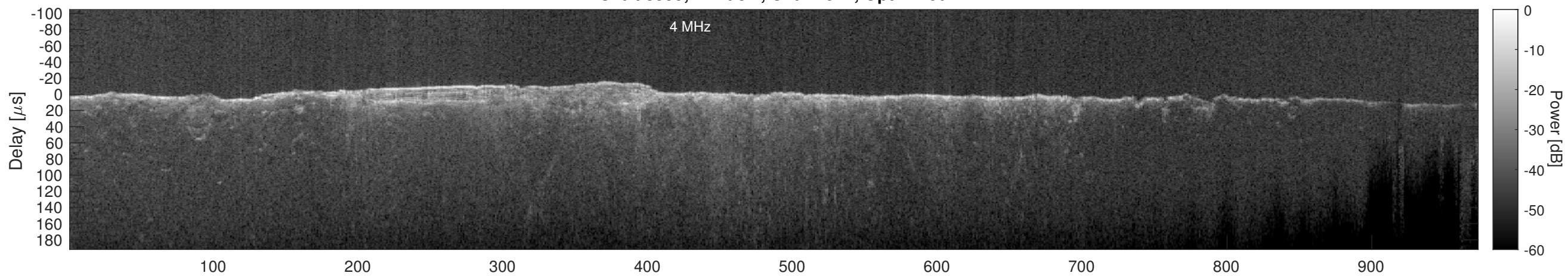
Orbit 8599, Cluttergram
