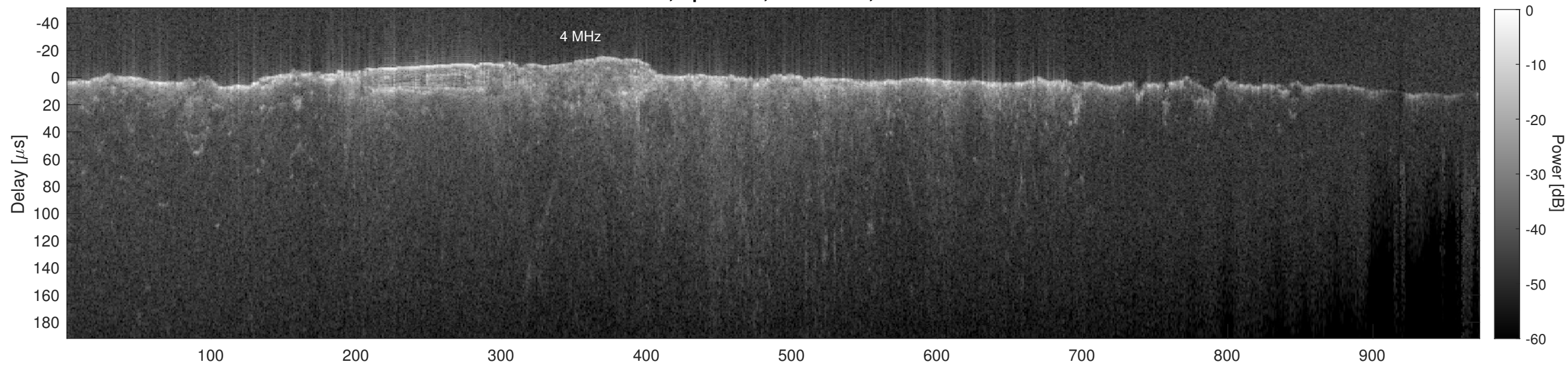
Orbit 8599, Cluttergram
