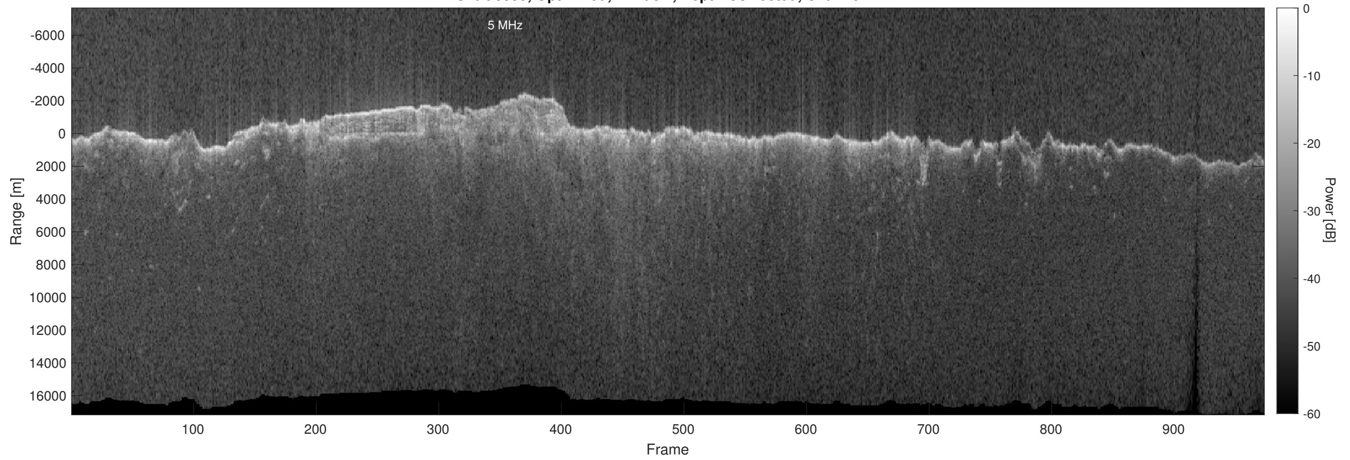
Orbit 8599, Optimized, Window, Depth-Corrected, Channel 2
