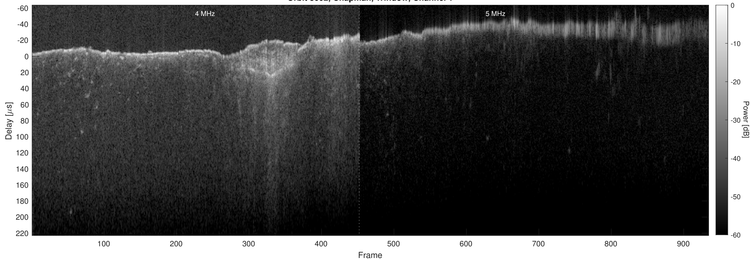
Orbit 8602, Chapman, Window, Channel 2
