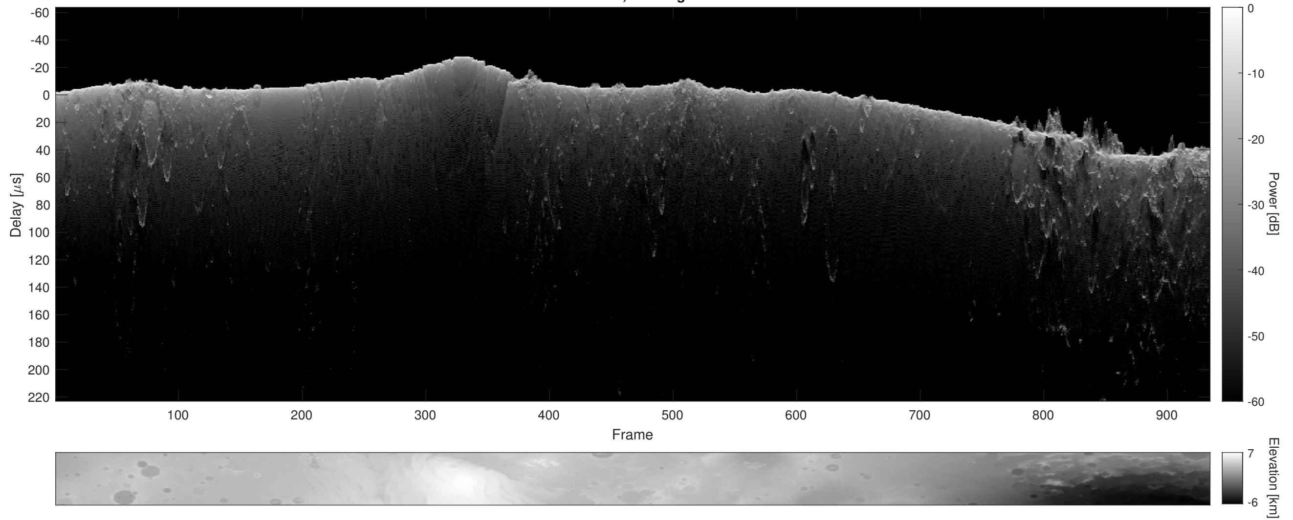
Orbit 8602, Cluttergram
