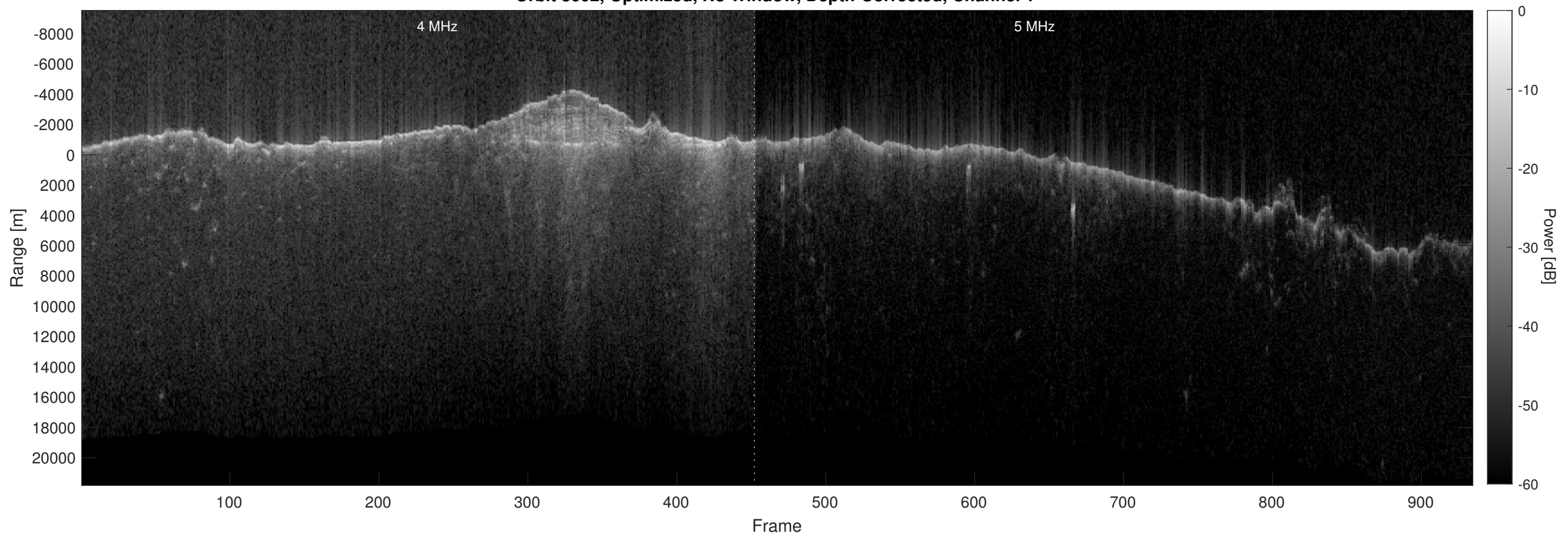
Orbit 8602, Optimized, No Window, Depth-Corrected, Channel 2
