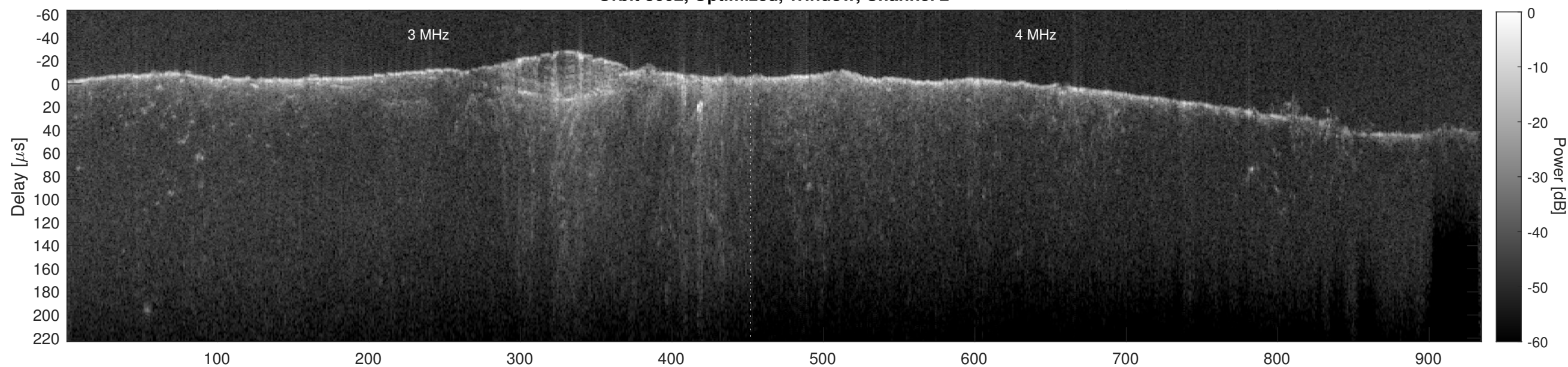
Orbit 8602, Cluttergram
