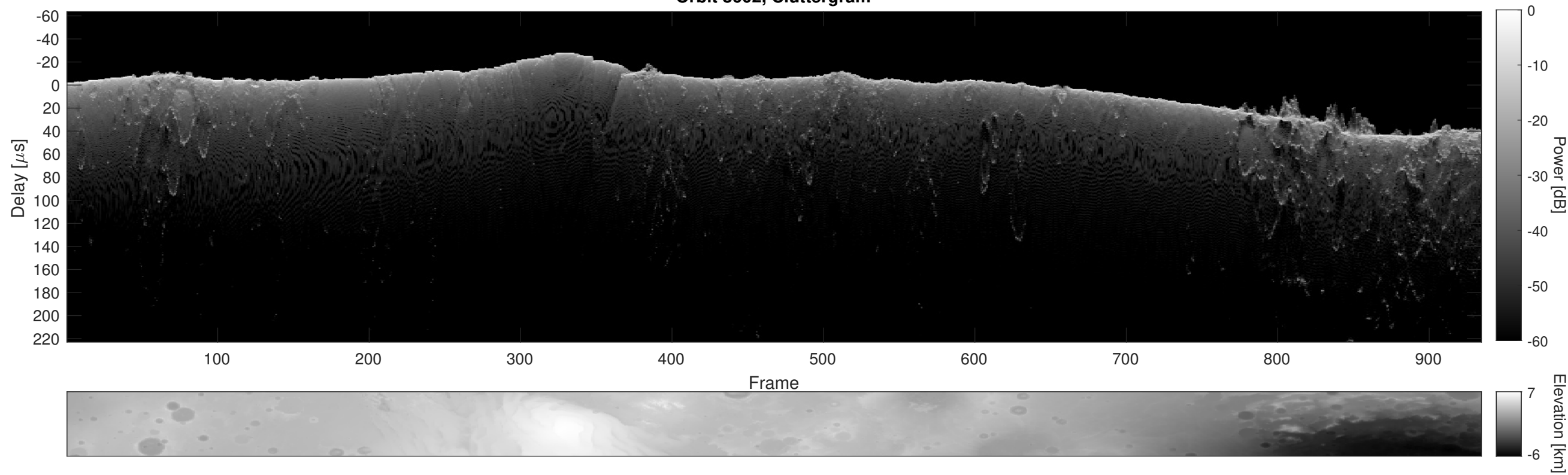
Orbit 8602, Cluttergram
