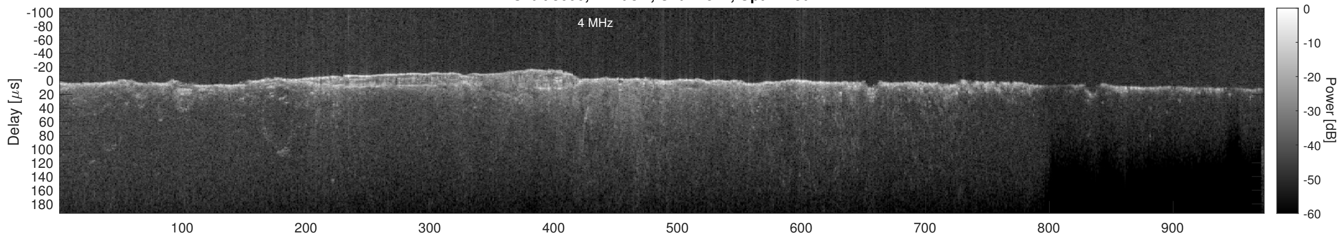
Orbit 8606, Cluttergram
