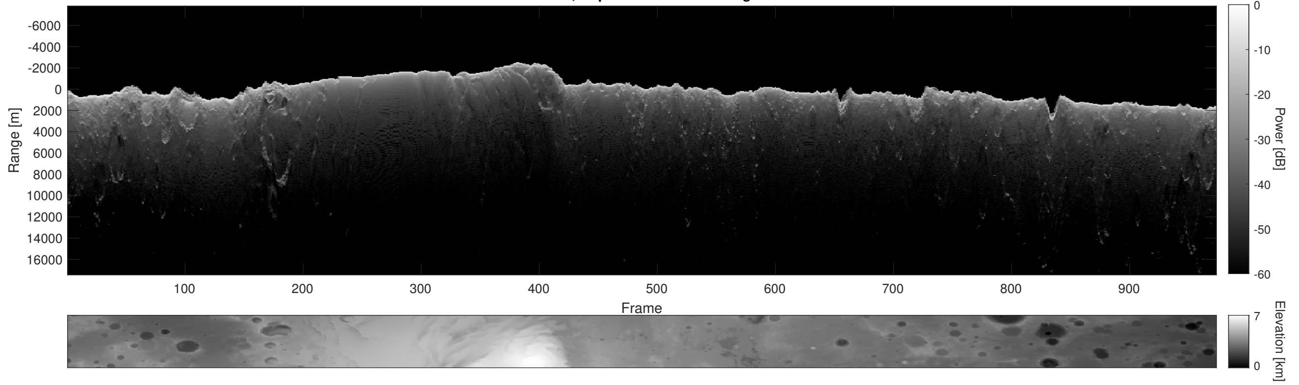
Orbit 8606, Depth-Corrected Cluttergram
