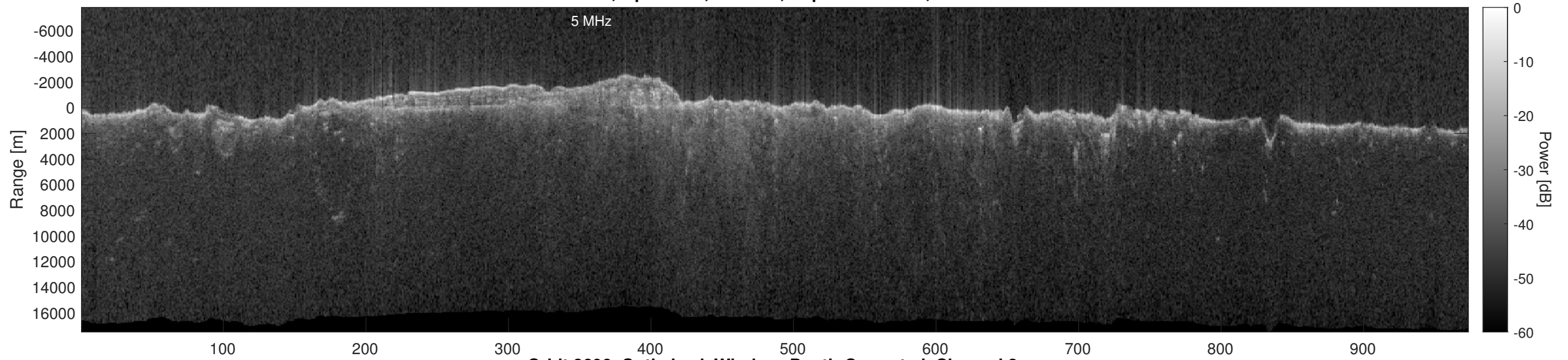
Orbit 8606, Optimized, Window, Depth-Corrected, Channel 2
