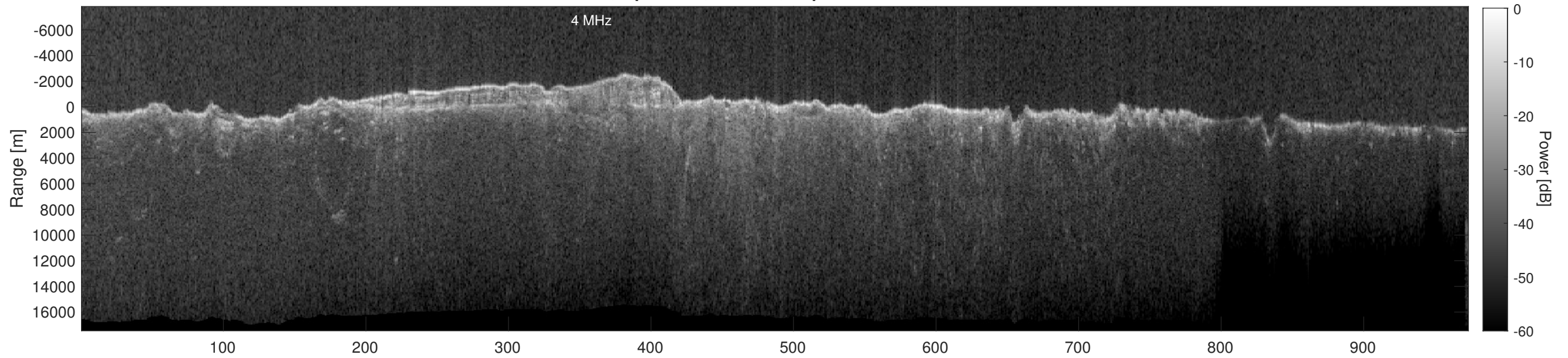
Orbit 8606, Depth-Corrected Cluttergram
