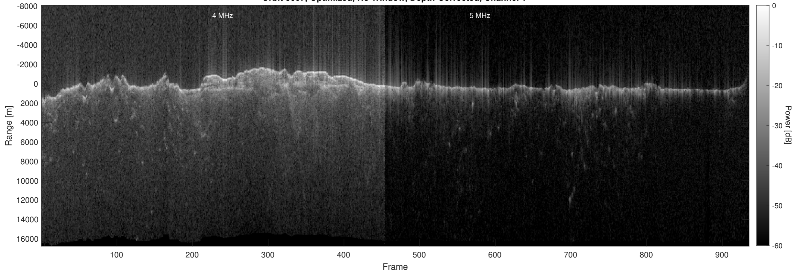
Orbit 8607, Optimized, No Window, Depth-Corrected, Channel 2
