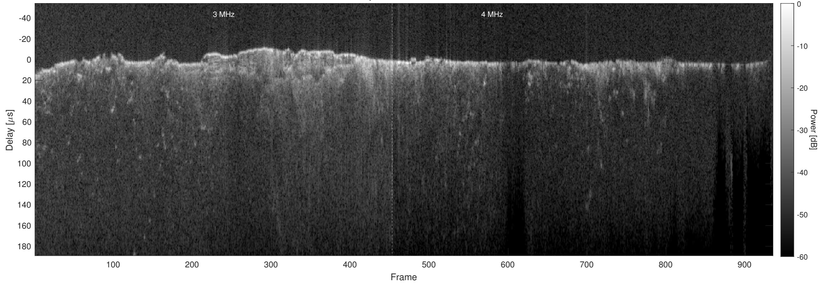
Orbit 8607, Optimized, Window, Channel 2
