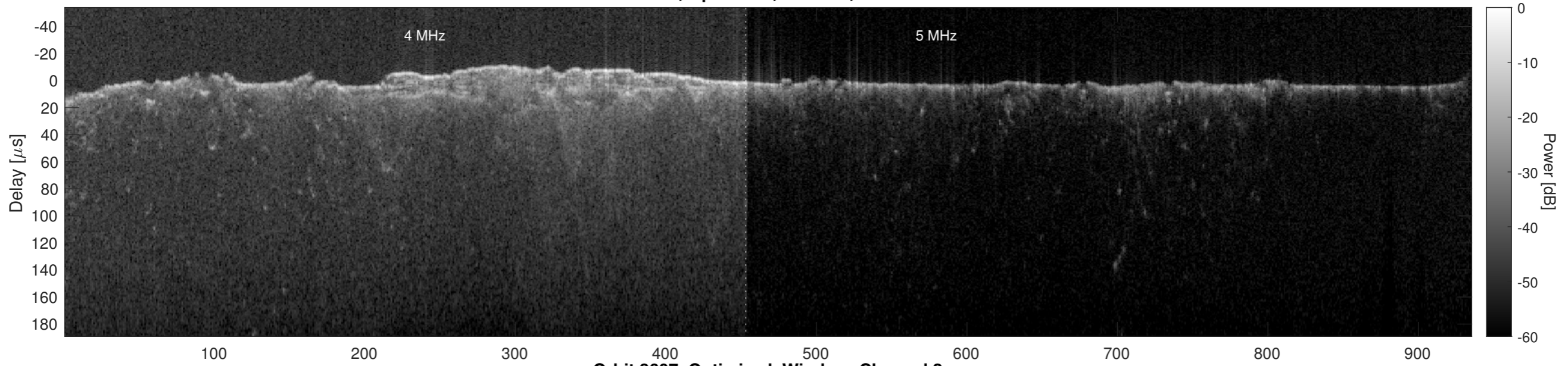
Orbit 8607, Optimized, Window, Channel 2
