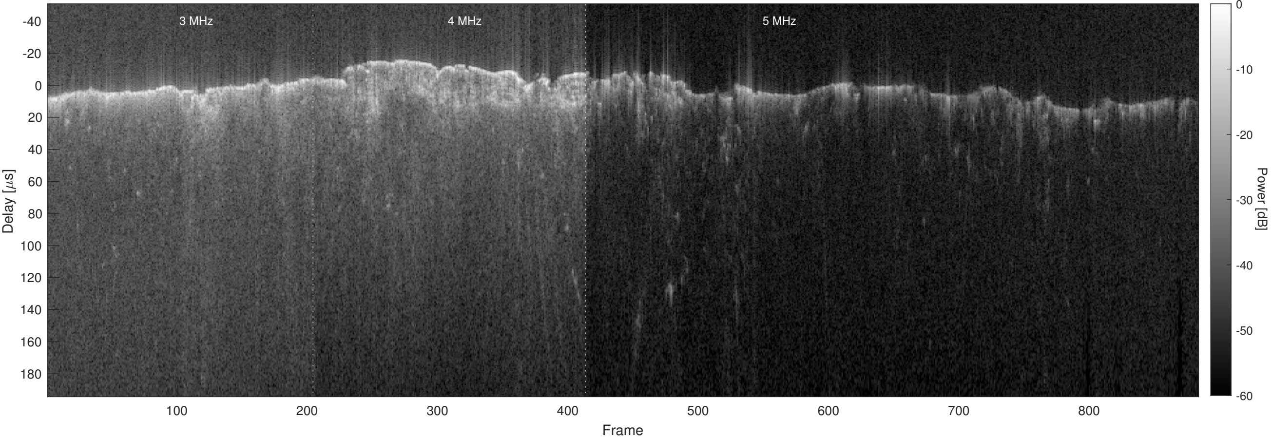
Orbit 8615, Optimized, No Window, Channel 2
