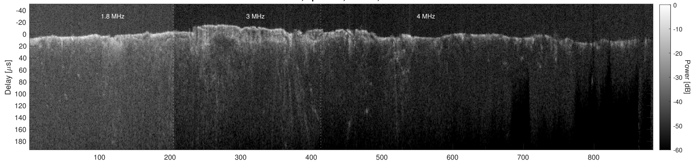
Orbit 8615, Cluttergram
