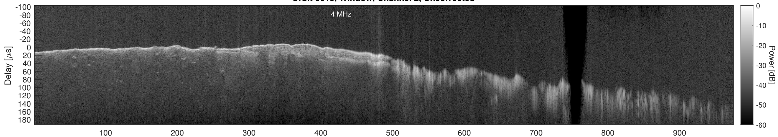
Orbit 8618, Window, Channel 2, Chapman
