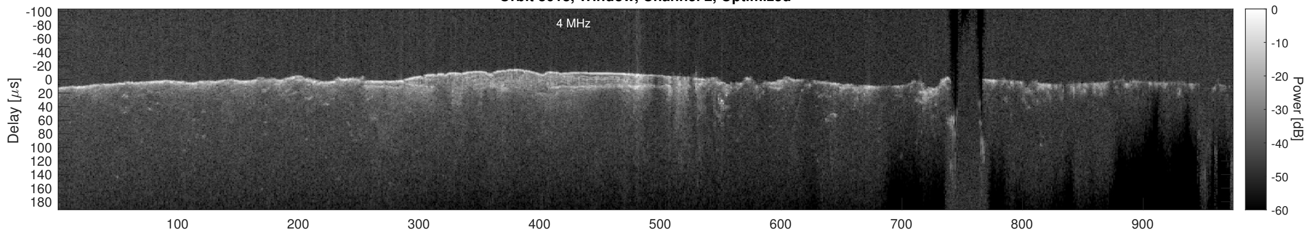
Orbit 8618, Cluttergram
