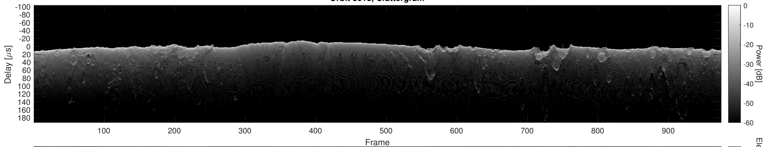
Orbit 8618, Cluttergram
