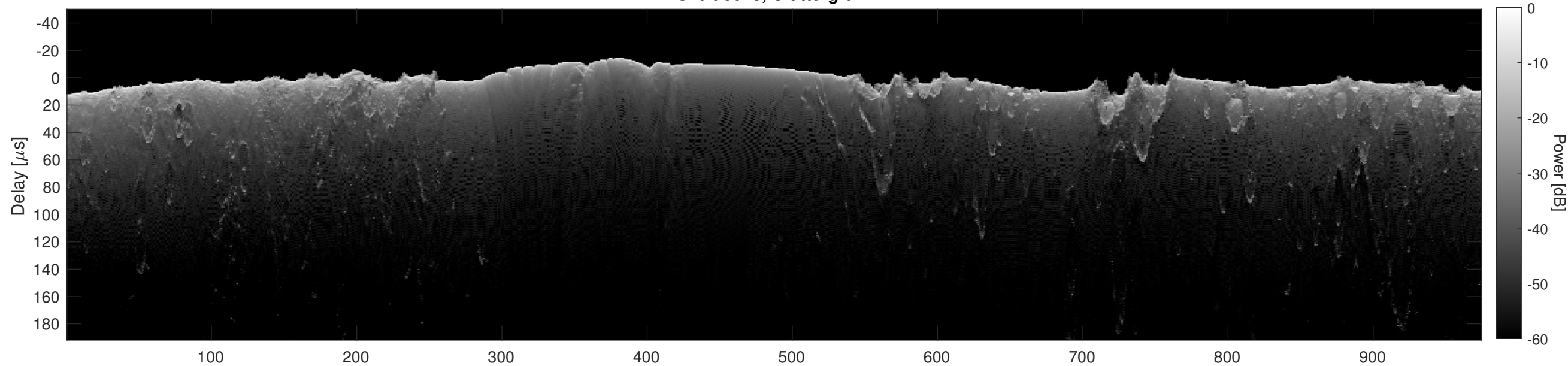
Orbit 8618, Cluttergram
