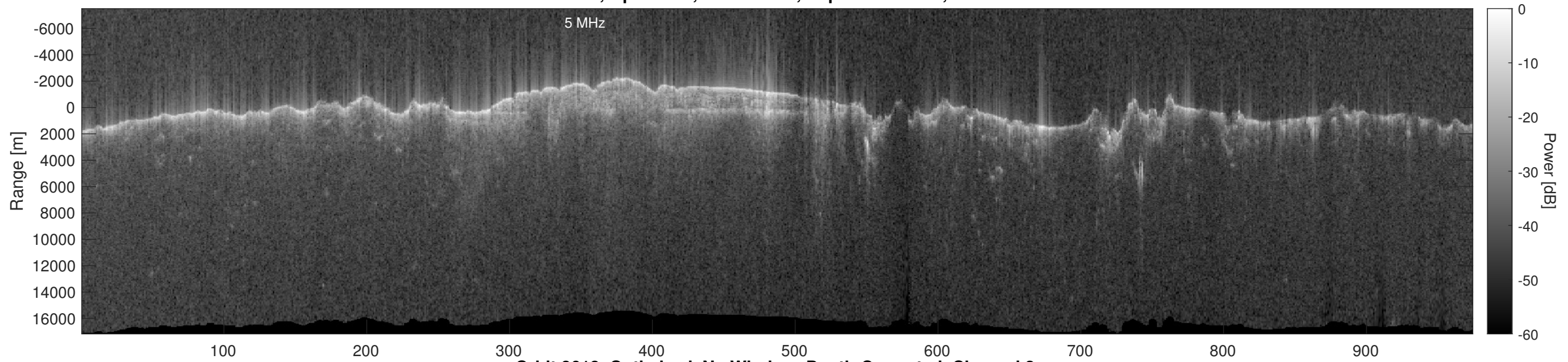
Orbit 8618, Optimized, No Window, Depth-Corrected, Channel 2
