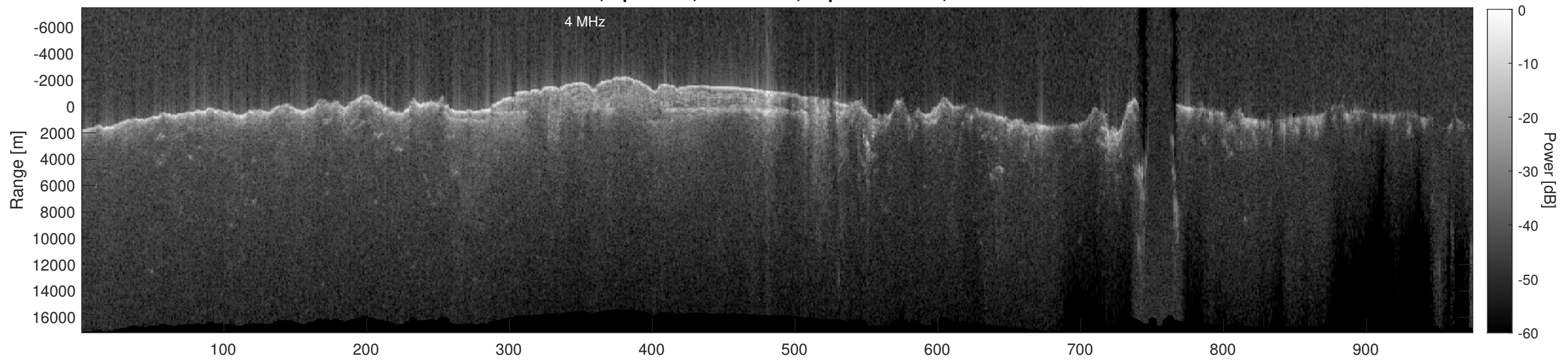
Orbit 8618, Depth-Corrected Cluttergram
