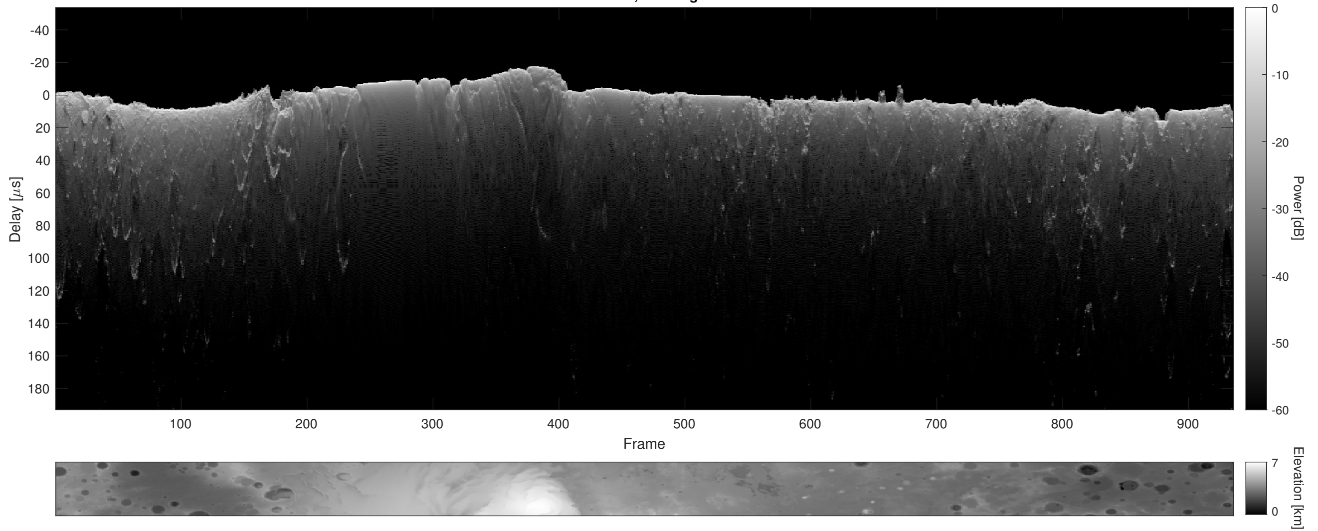
Orbit 8620, Cluttergram
