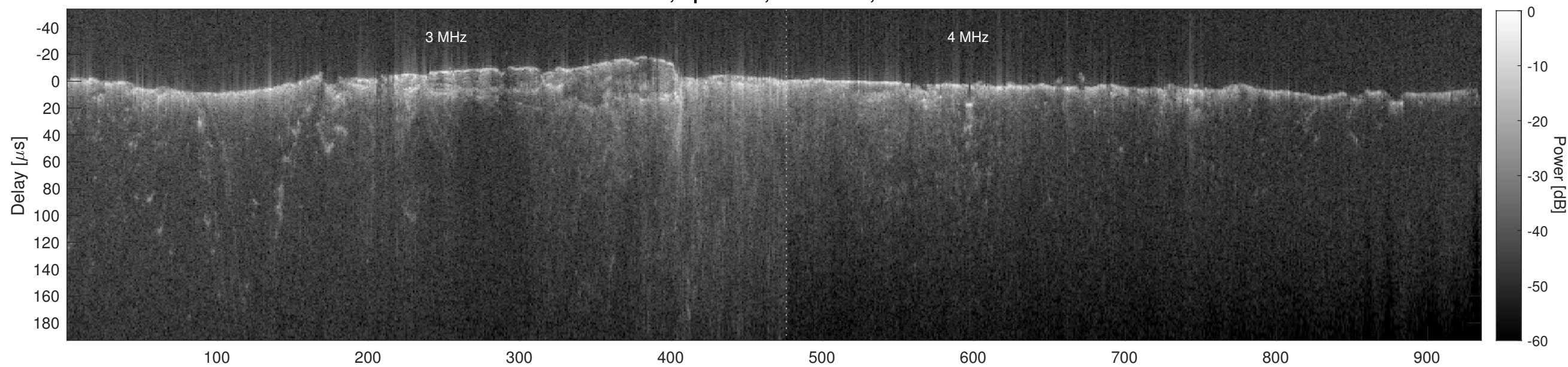
Orbit 8620, Cluttergram
