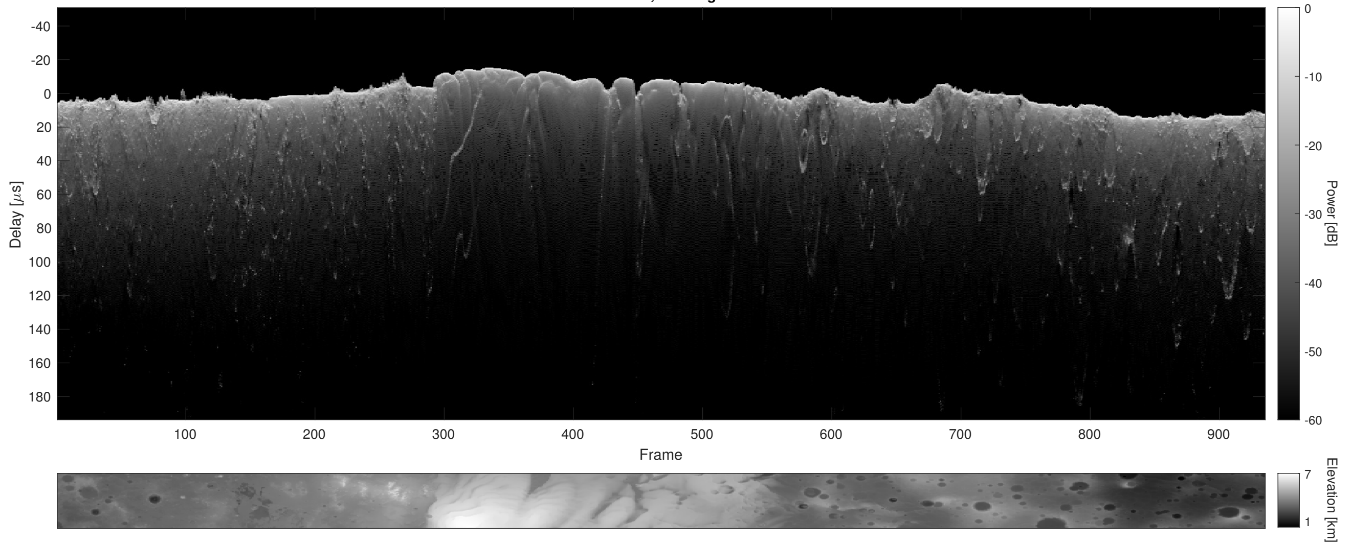
Orbit 8622, Cluttergram
