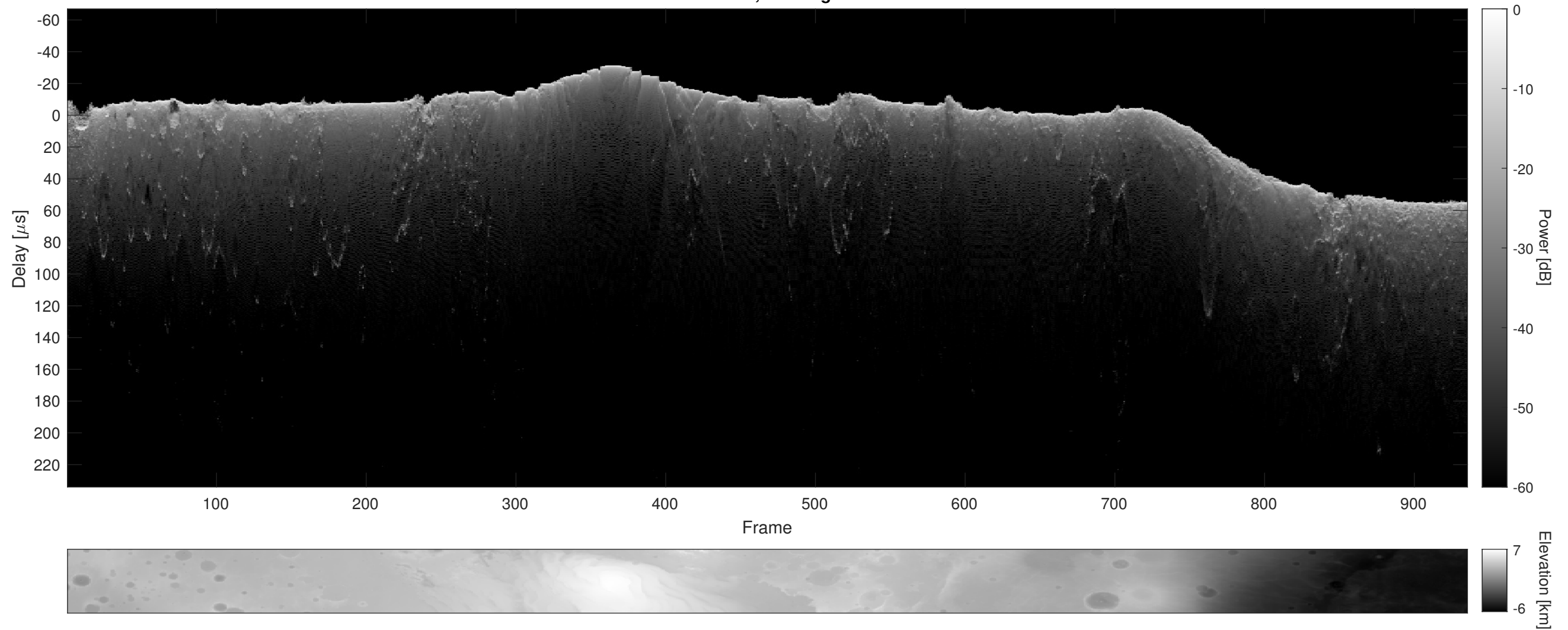
Orbit 8623, Cluttergram
