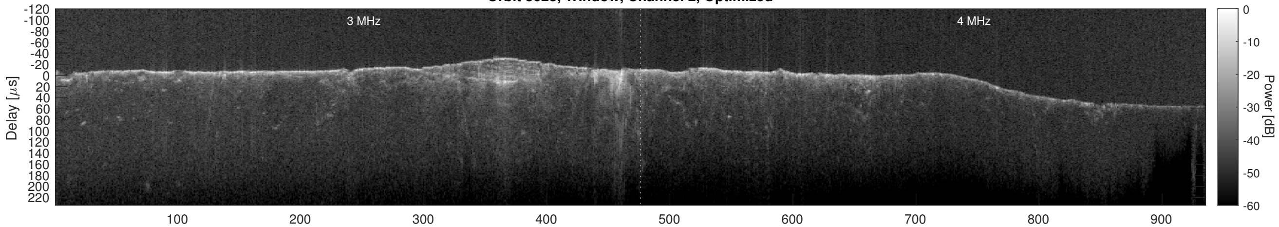
Orbit 8623, Cluttergram
