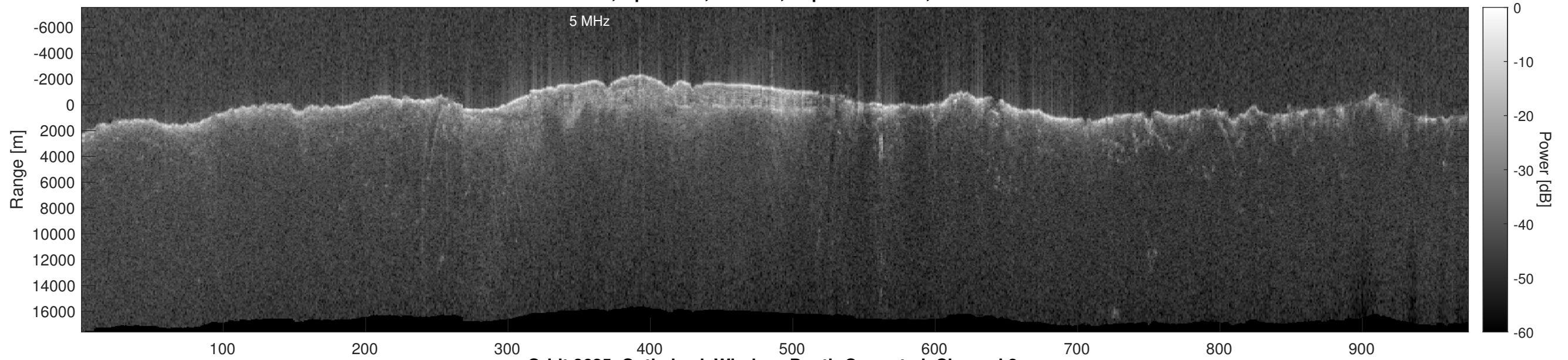
Orbit 8625, Optimized, Window, Depth-Corrected, Channel 2
