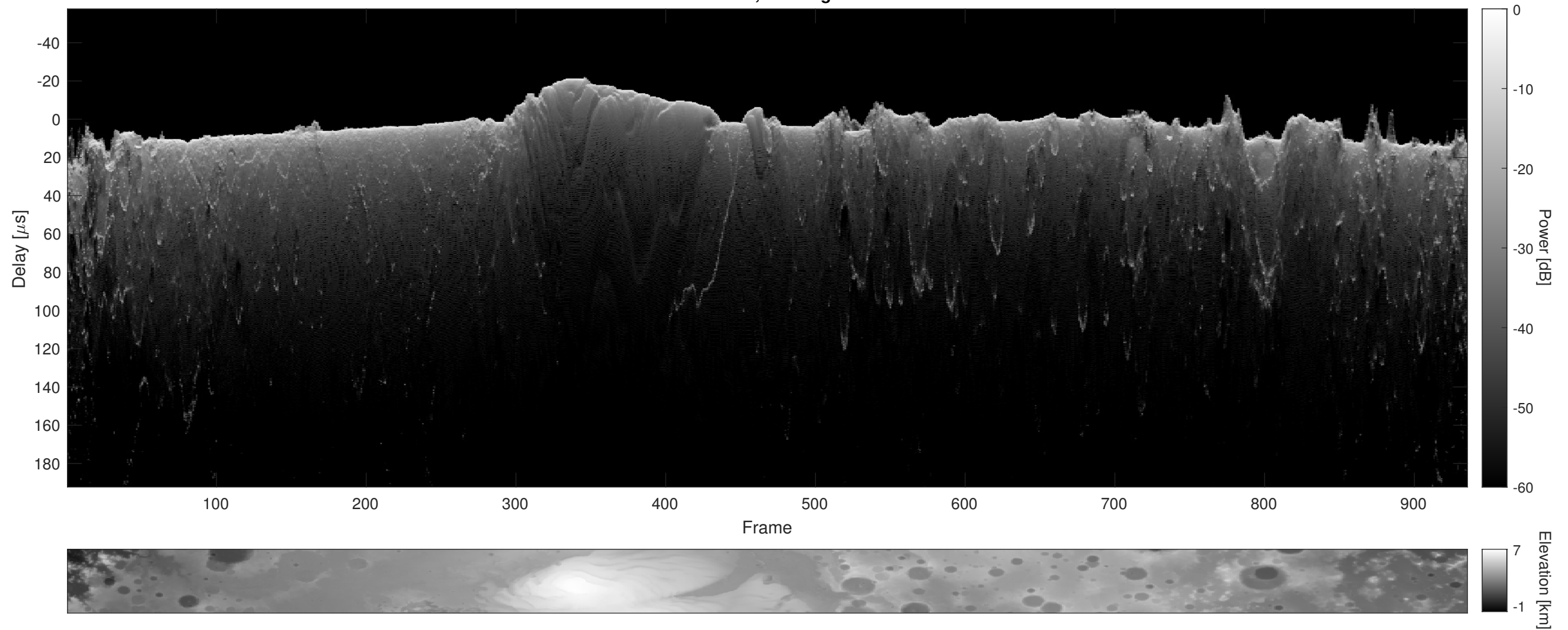
Orbit 8626, Cluttergram
