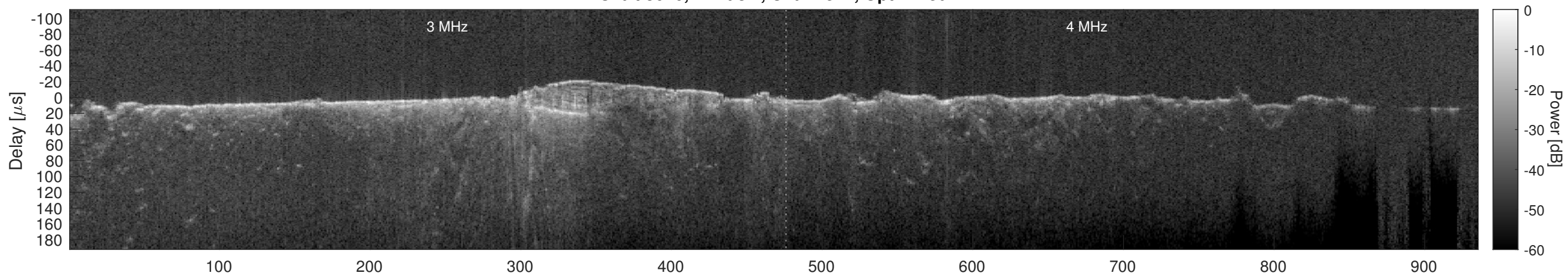
Orbit 8626, Cluttergram
