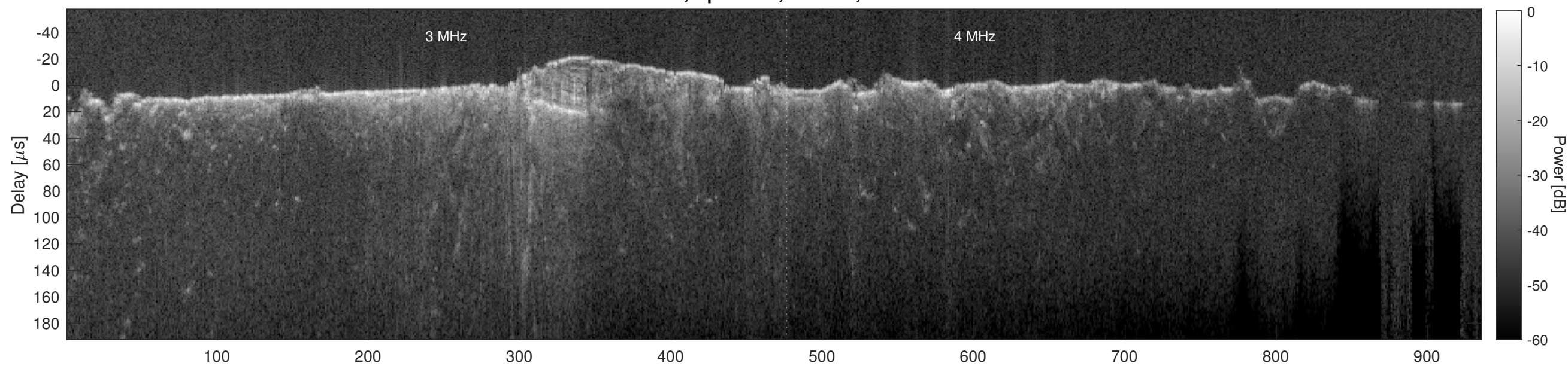
Orbit 8626, Cluttergram
