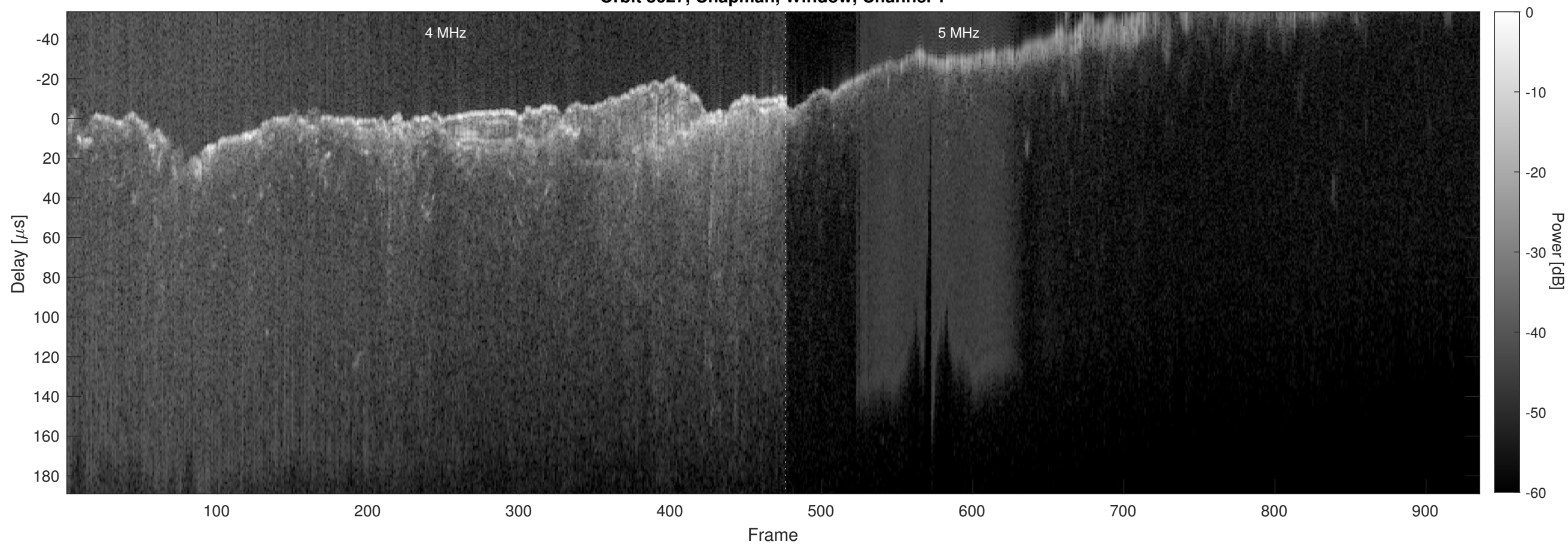
Orbit 8627, Chapman, Window, Channel 2
