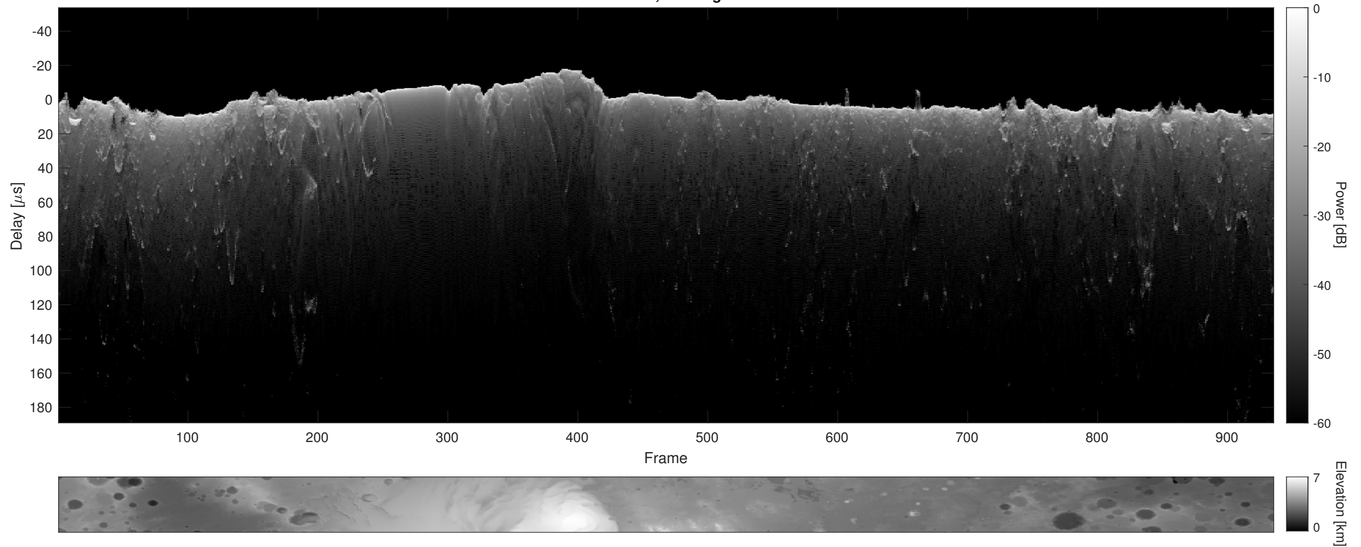
Orbit 8627, Cluttergram
