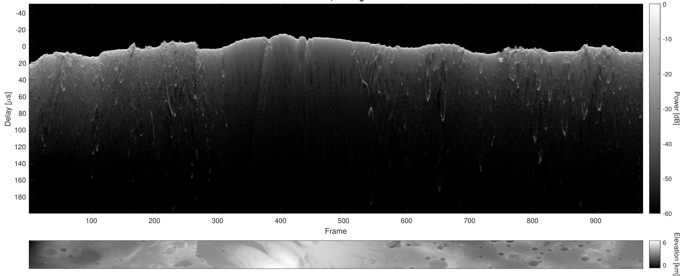
Orbit 8632, Cluttergram
