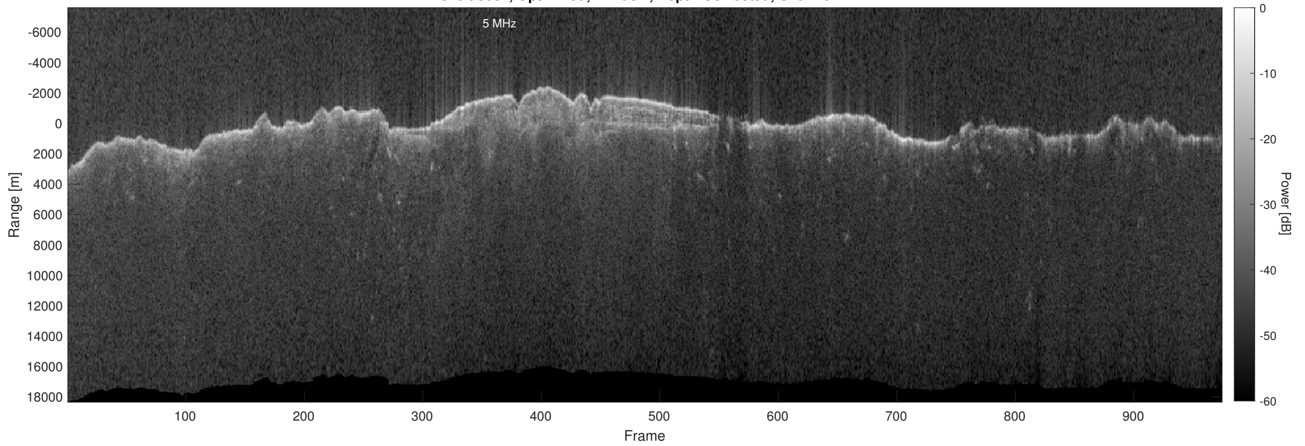
Orbit 8632, Optimized, Window, Depth-Corrected, Channel 2
