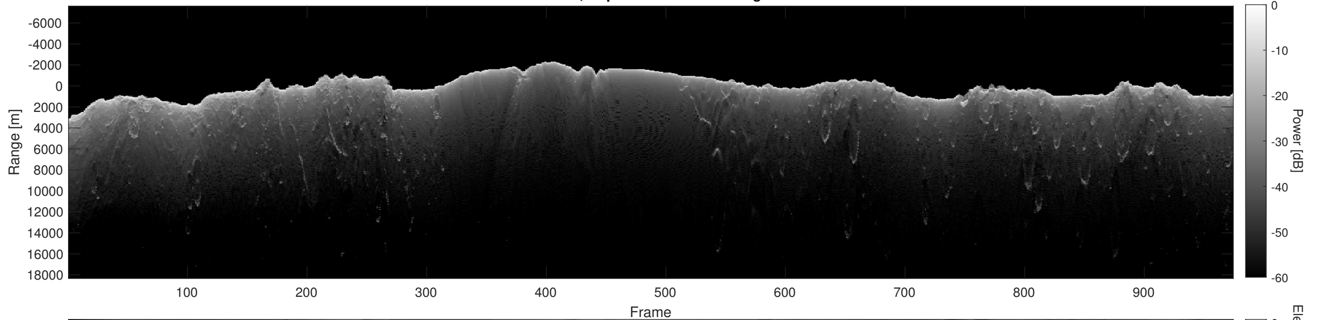
Orbit 8632, Depth-Corrected Cluttergram
