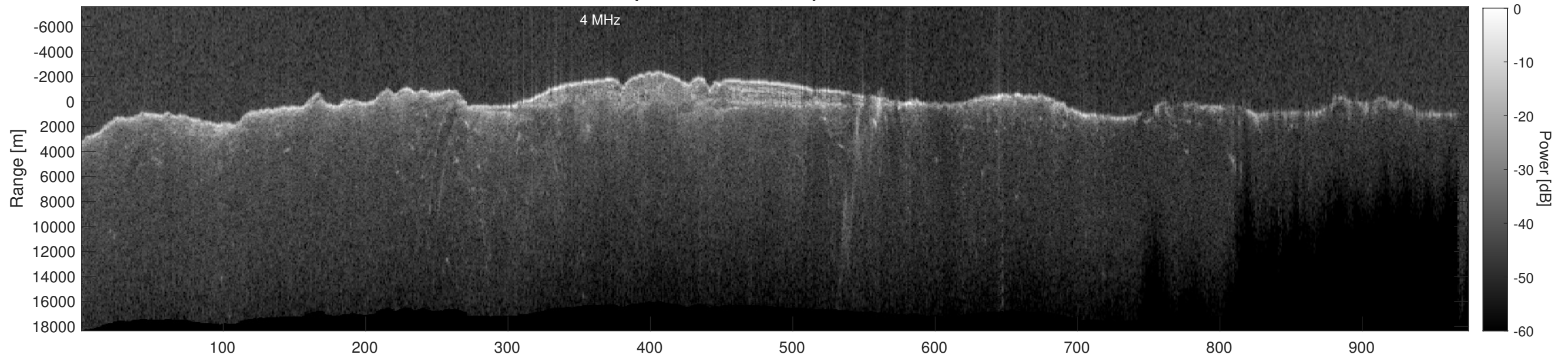
Orbit 8632, Depth-Corrected Cluttergram
