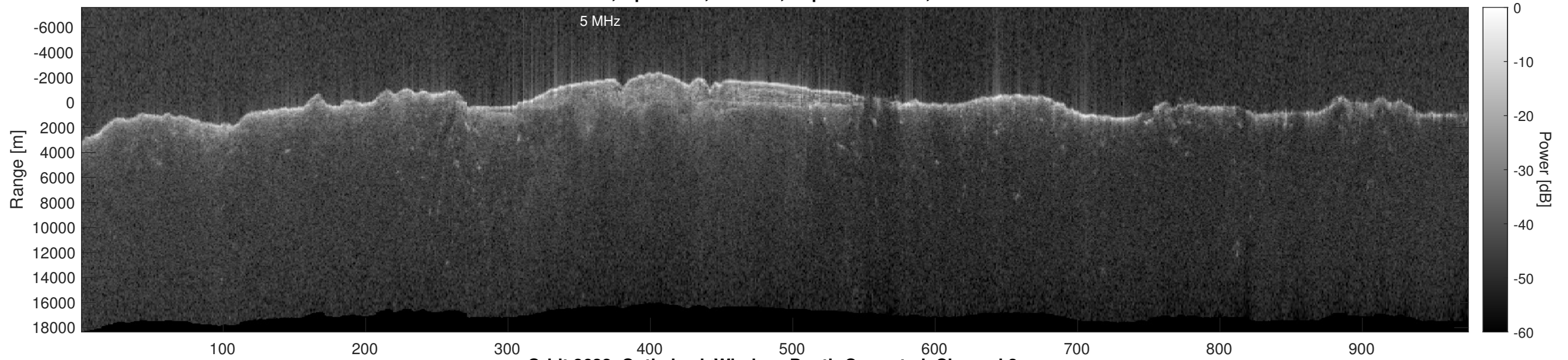
Orbit 8632, Optimized, Window, Depth-Corrected, Channel 2
