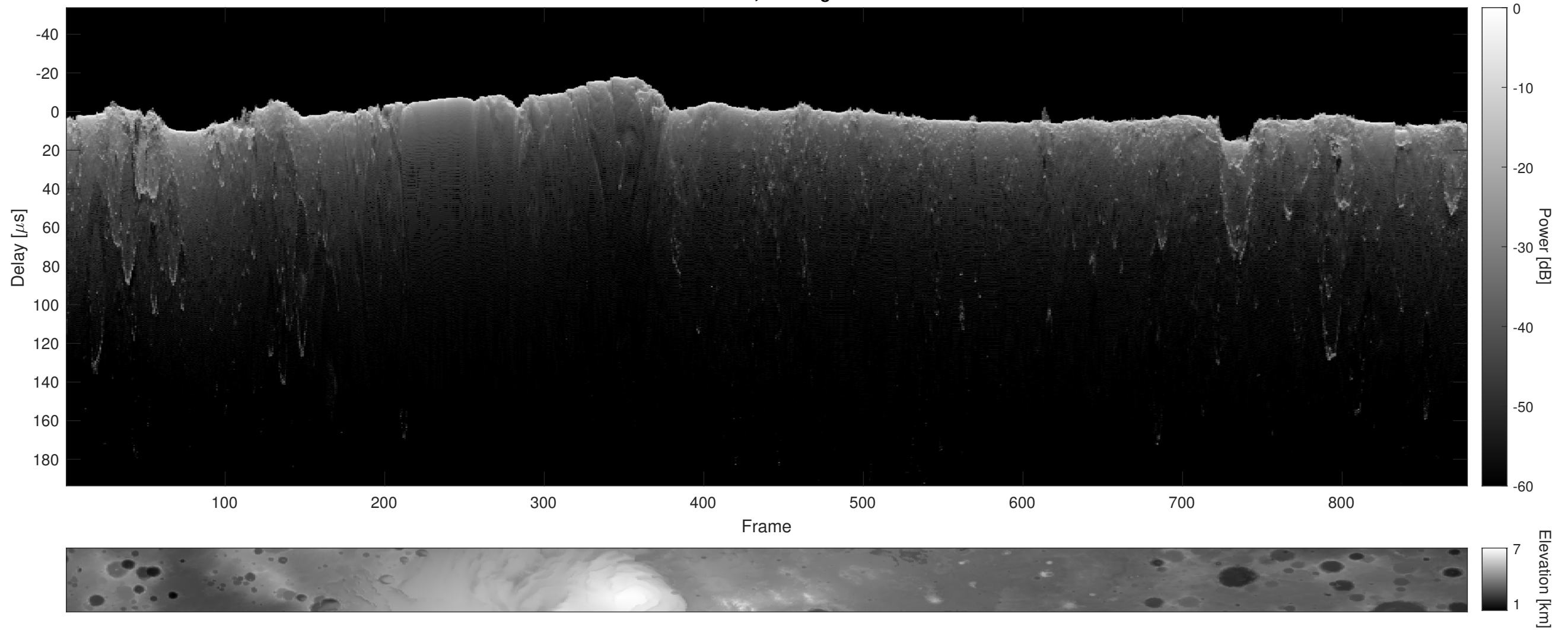
Orbit 8634, Cluttergram
