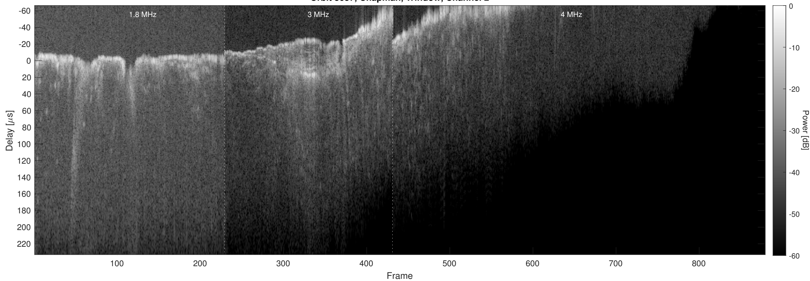
Orbit 8637, Chapman, Window, Channel 2
