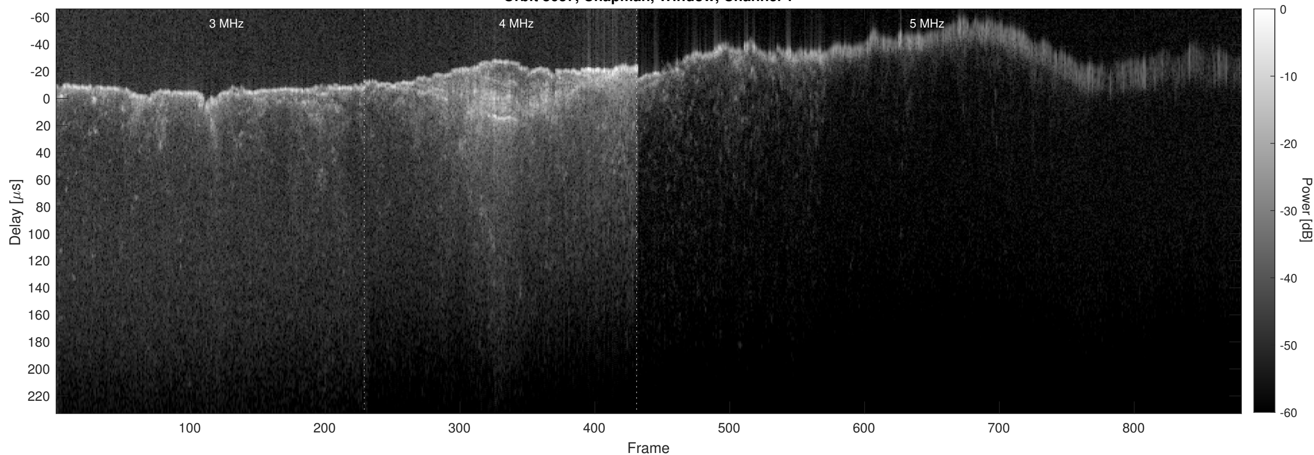
Orbit 8637, Chapman, Window, Channel 2
