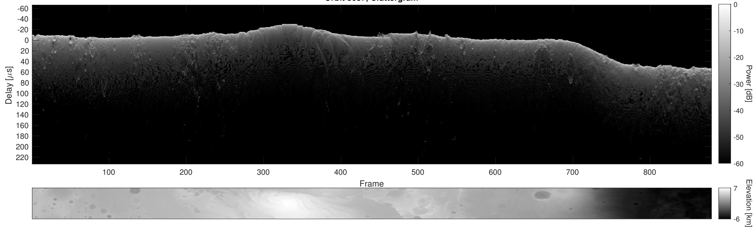
Orbit 8637, Cluttergram
