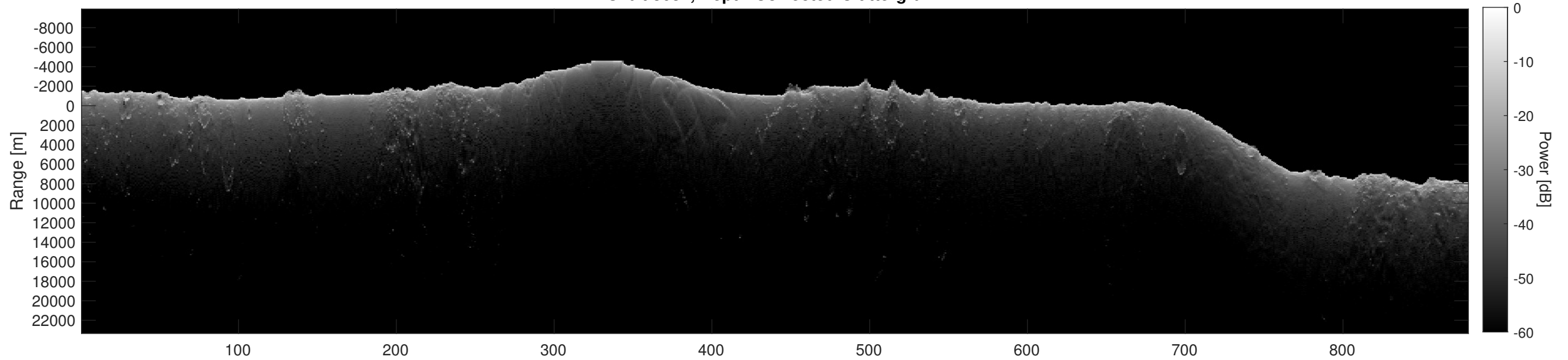
Orbit 8637, Depth-Corrected Cluttergram
