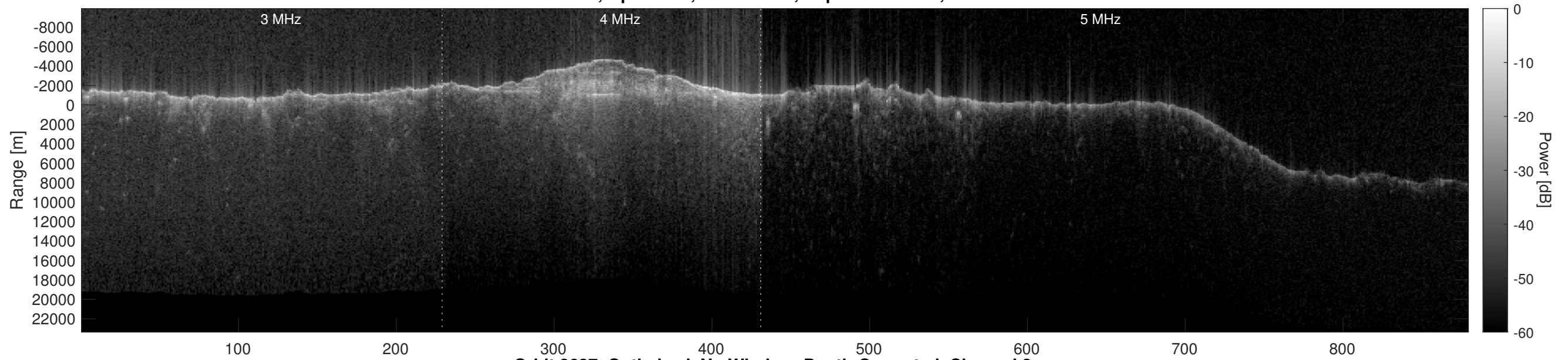
Orbit 8637, Optimized, No Window, Depth-Corrected, Channel 2
