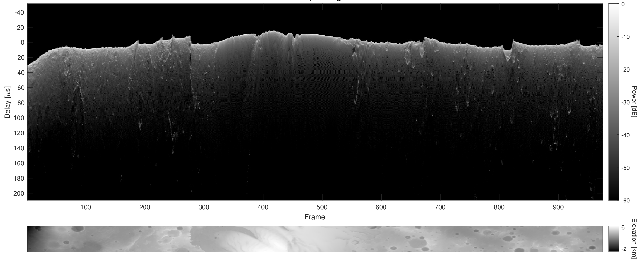
Orbit 8639, Cluttergram
