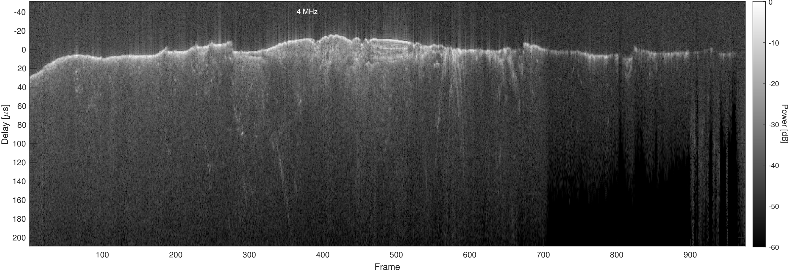
Orbit 8639, Optimized, No Window, Channel 2
