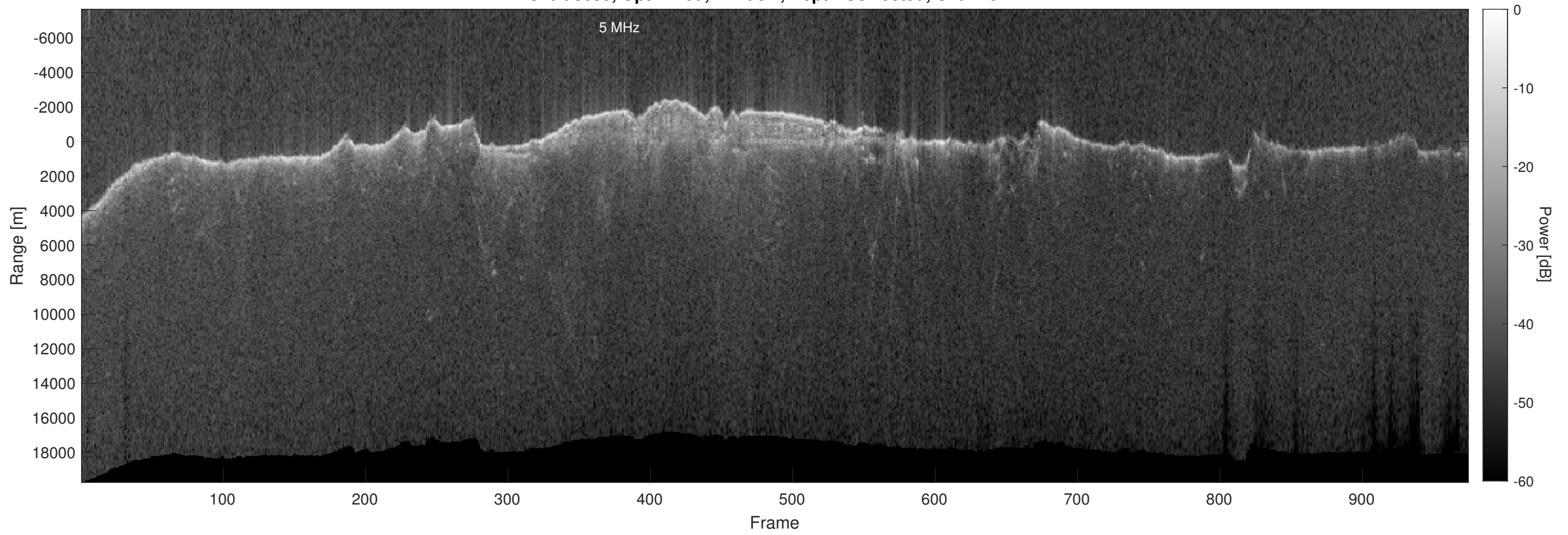
Orbit 8639, Optimized, Window, Depth-Corrected, Channel 2
