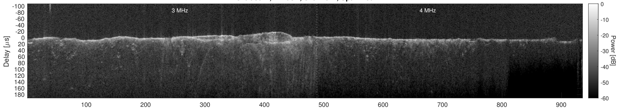
Orbit 8641, Cluttergram
