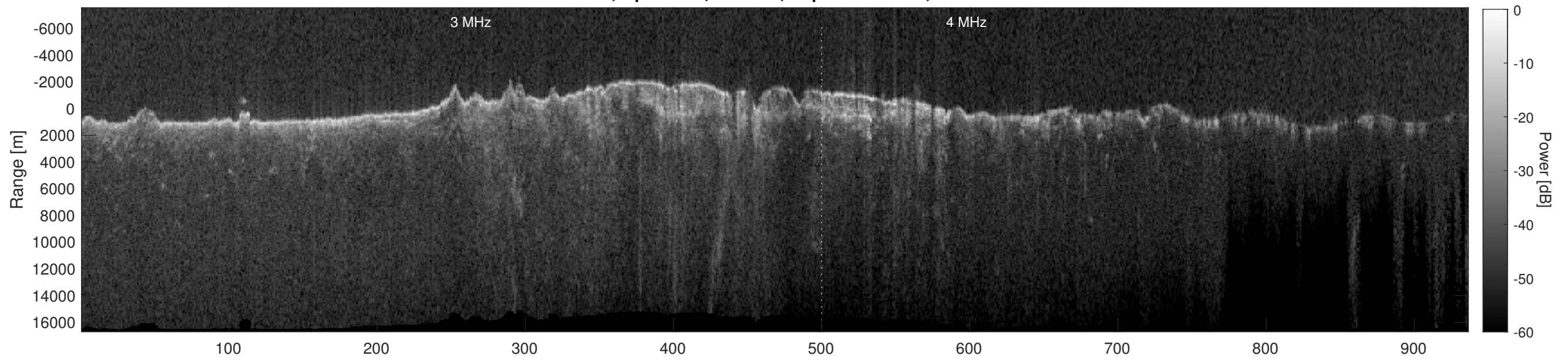
Orbit 8643, Depth-Corrected Cluttergram
