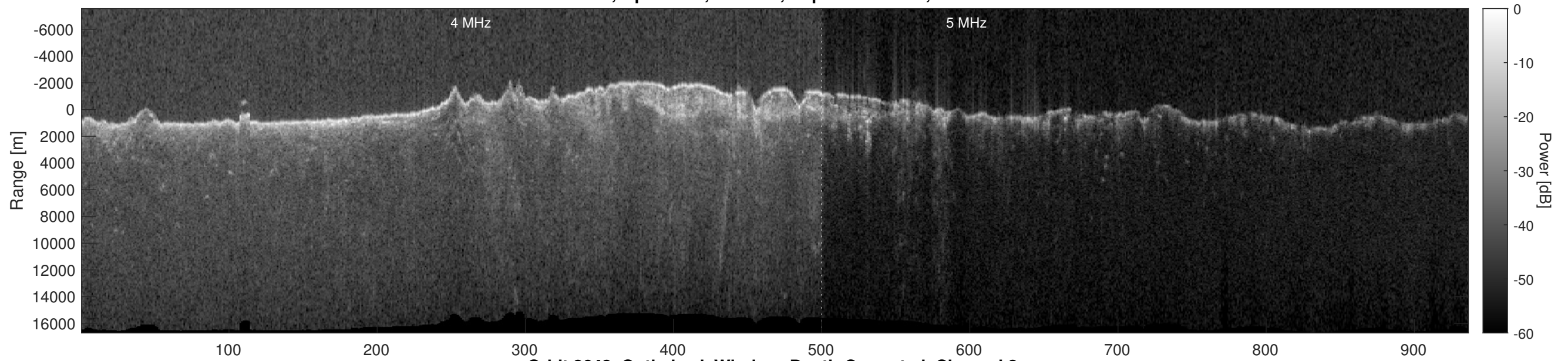
Orbit 8643, Optimized, Window, Depth-Corrected, Channel 2
