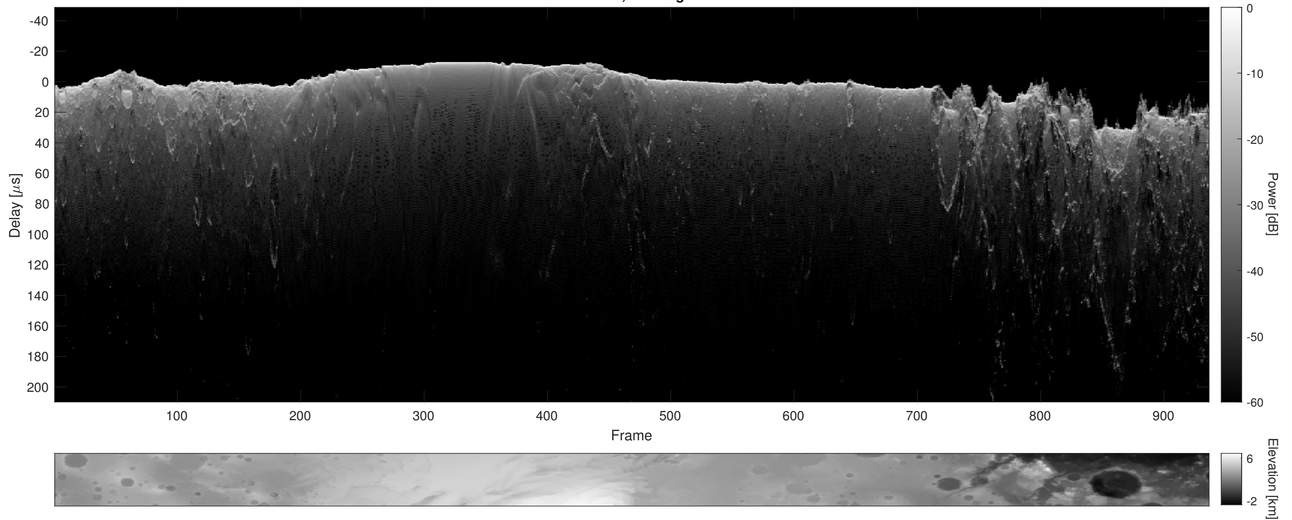
Orbit 8645, Cluttergram
