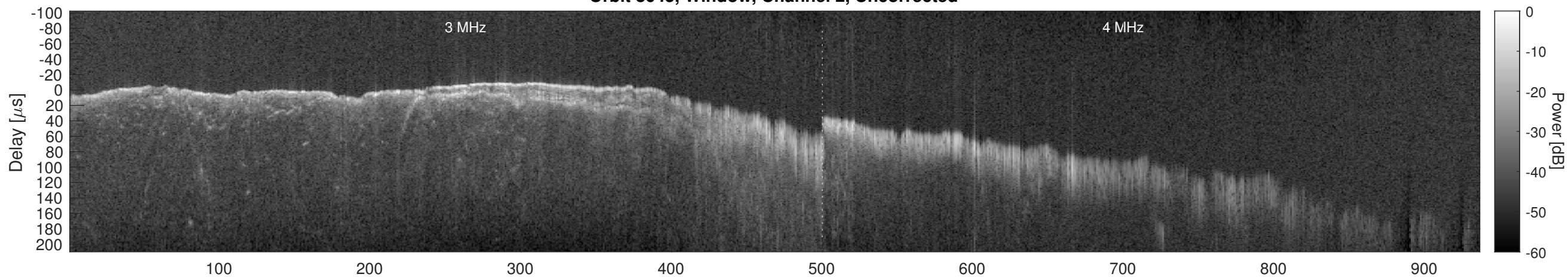
Orbit 8645, Window, Channel 2, Chapman
