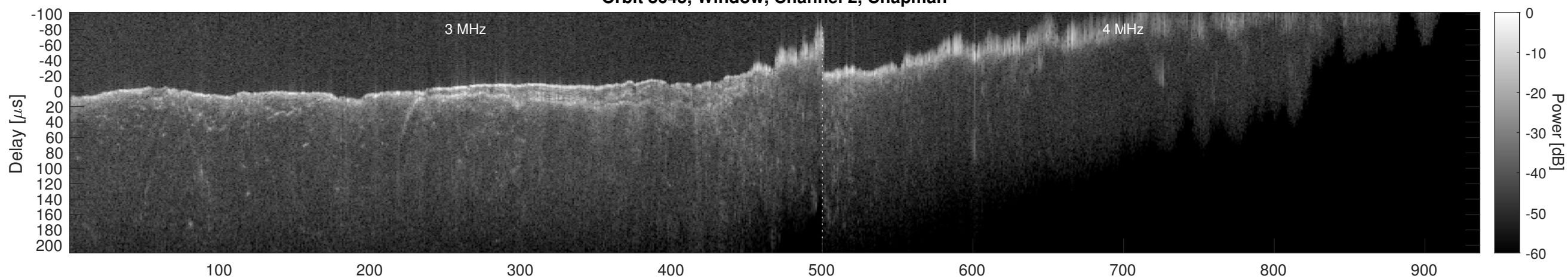
Orbit 8645, Window, Channel 2, Optimized
